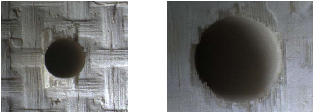
Figure 37: Pre-test optical micrographs of N720/A specimens with diamond-drilled holes showing material in the vicinity of randomly selected holes
