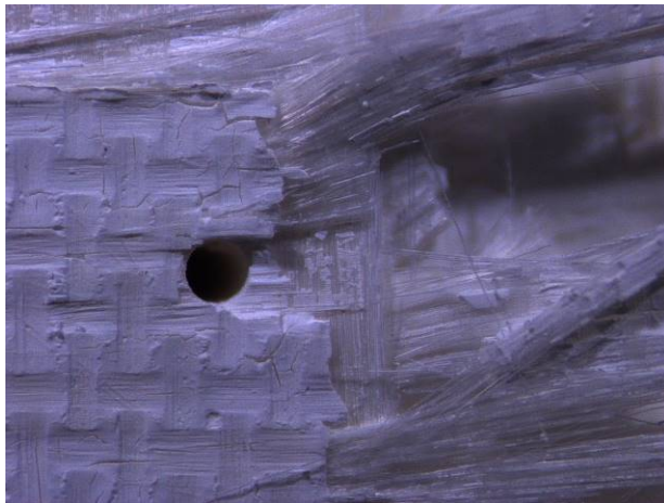
Figure A. 10: Fracture surface of specimen #3, tested in tension to failure at 1200°C in air
