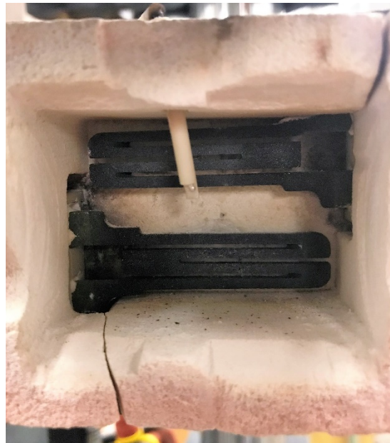
Figure 11: Interior view of insulated furnace with heating elements and control thermocouple
