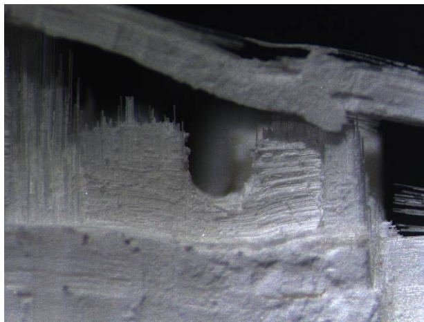
Figure A. 23: Fracture surface of specimen #6, tested in creep at 1200°C in air ( \sigma_{cr} = 69 MPa, t_f = 30.95 h)
