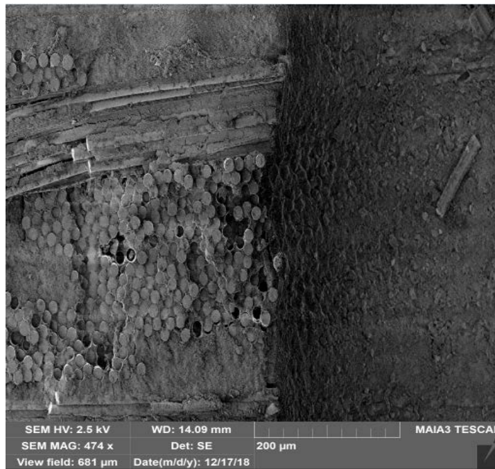
Figure 52: Fracture surface of an N720/A specimen with diamond-drilled holes tested in creep at 1200°C in steam ( \sigma_{cr} = 93 MPa, t_f = 6.05 h)
